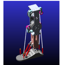
Motor – String System
